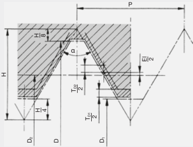
Profile of the internal thread
