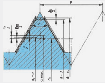
Profile of the tap
